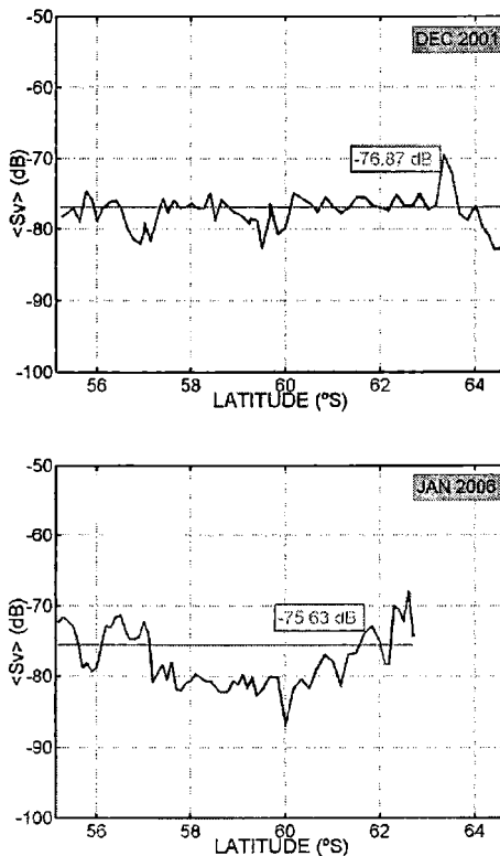
Figure 9. Averaged \langle S_v \rangle along the water column depth-layer between: (a) 26 m and 154 m, on transect made during Event I. Latitude-averaged S_{va} = -76.87 dB; (b) 22 m and 150 m, on transect made during Event II. Latitude-averaged S_{va} = -75.63 dB.
