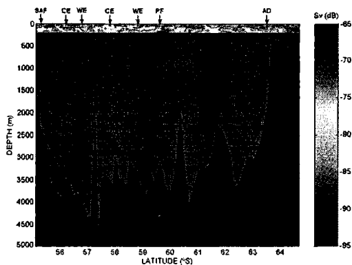
Figure 8. Superposition of the bathymetry with the computed Volume Backscattering Strengths (dB) vs. depth (m) and latitude (°S) for Event I.
